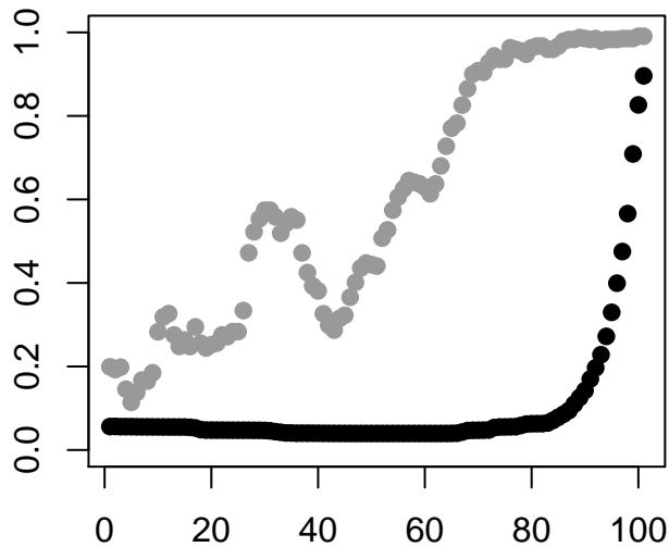
Conservation Per Base 100bp Upstream (Control Black, Alt Gray)
