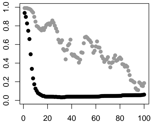
Conservation Per Base 100bp Downstream (Control Black, Alt Gray)
