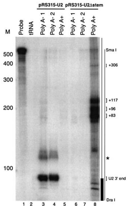
Fig. 6. Deletion of the Rnt1 cleavage sites leads to polyadenylation of U2 snRNA. Total RNA extracted from pRS315-U2 (lanes 3–5) or pRS315-U2Δstem cells (lanes 6–8) was fractionated on oligo(dT)-cellulose, and both poly(A) - ('flow-through', poly A - 1, lanes 3 and 6; 'first wash', lanes 4 and 7) and poly(A) + RNA fractions (lanes 4 and 8) were subjected to the RNase protection assay as in Figure 5. The mature U2 3' end and the ends of the extended forms are indicated by brackets on the right. The numbering of positions of the extended forms is indicated using the wild-type U2 sequence. The asterisk indicates cleavage due to sequence divergence between the U2Δstem probe and transcripts from the wild-type U2 gene. Undigested probe (lane 1) and probe digested after hybridization to tRNA (lane 2) are included as controls.
